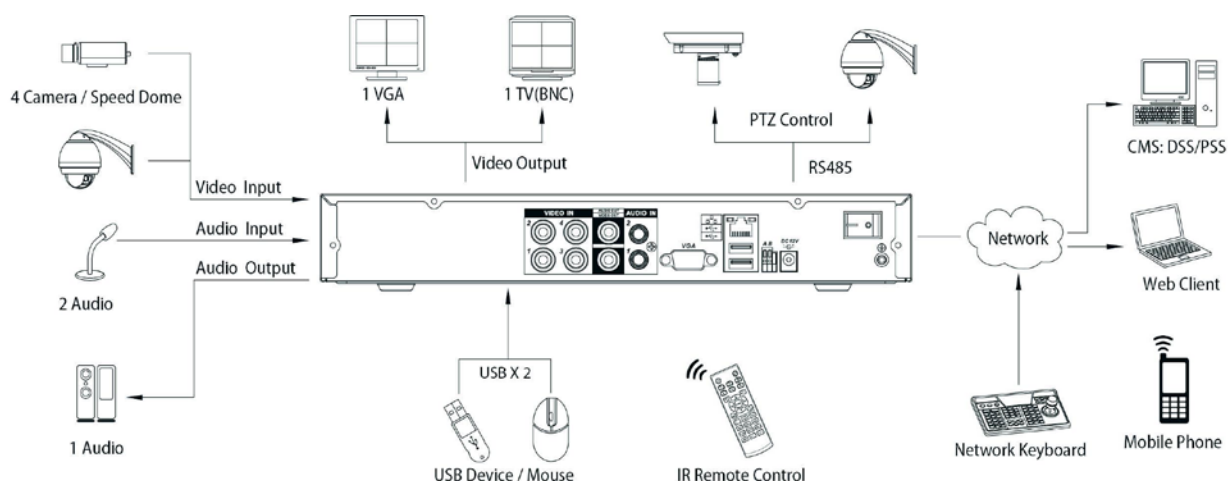
DVR3104SystemConnection
