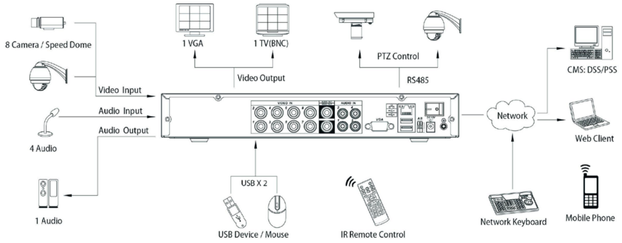
DVR3108SystemConnection
