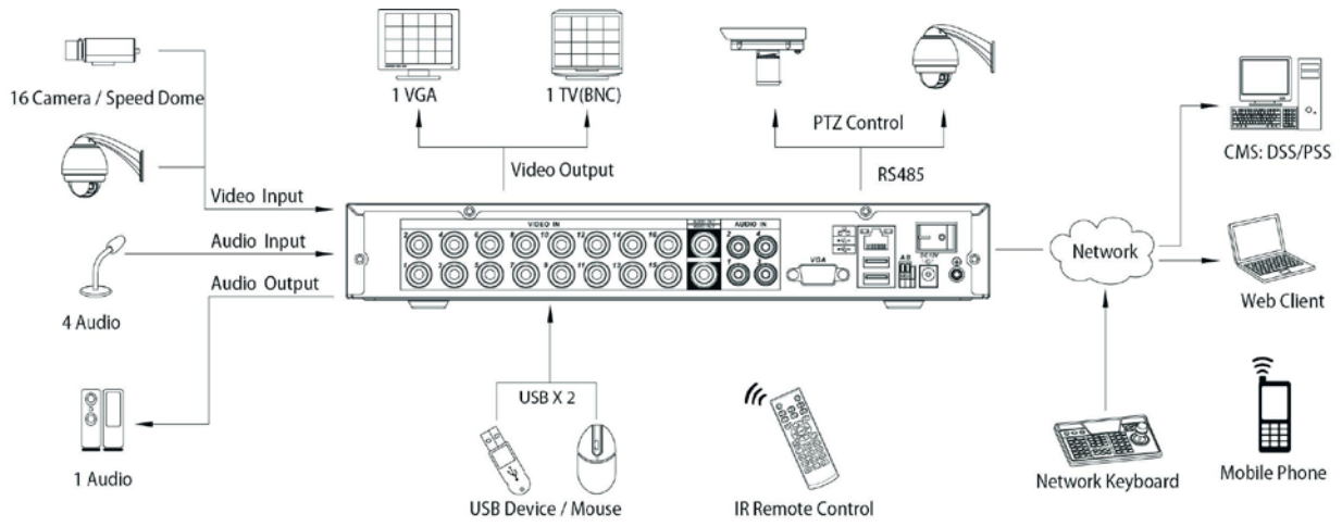
DVR3116 SystemConnection
